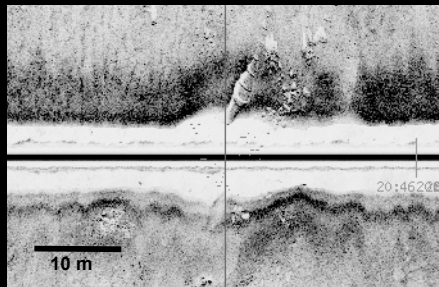
Scour around pipelines
